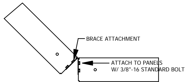
45 DEG DETAIL
