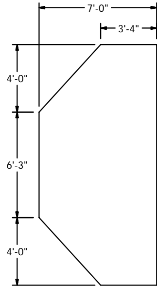
45 DEG DETAIL
