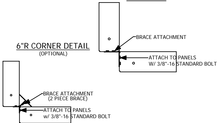
90° CORNER DETAIL OPTIONAL
