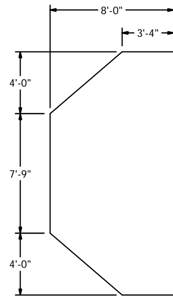
90° CORNER DETAIL OPTIONAL
