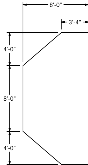
90° CORNER DETAIL OPTIONAL
